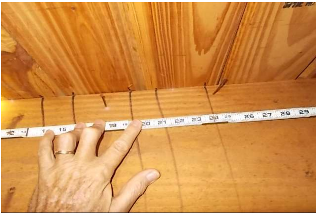
Nailing pattern
